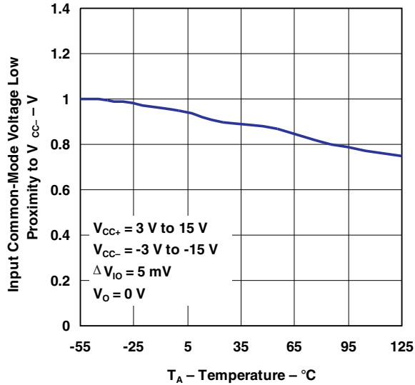
INPUT COMMON-MODE VOLTAGE LOW PROXIMITY TO V_{CC-} VS TEMPERATURE
